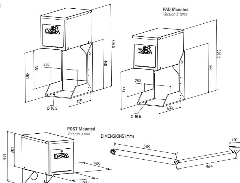
12711205 "C" shaped plate for pad mounting Plaque de fixation au sol
