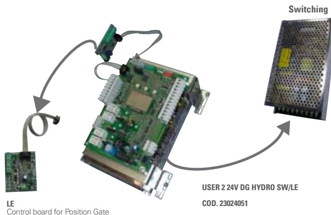
LE Control board for Position Gate
