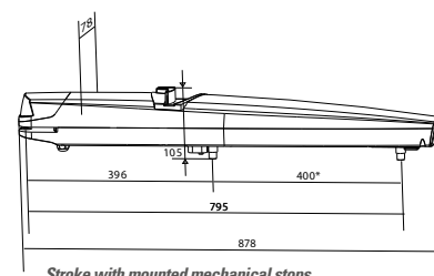
Stroke with mounted mechanical stops
