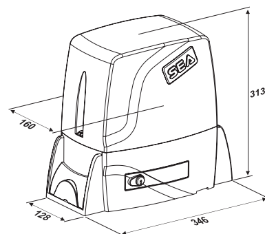
DIMENSIONS (mm)
