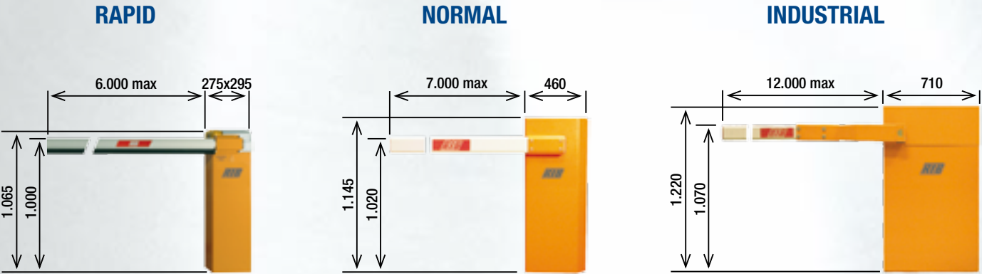
Misure in mm - Measurements in mm - Medidas en mm - Abmessungen in mm
