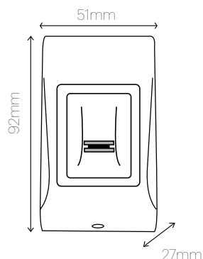
bx Black Edition Ref: B100PBK-RS-EH Black - ABS
