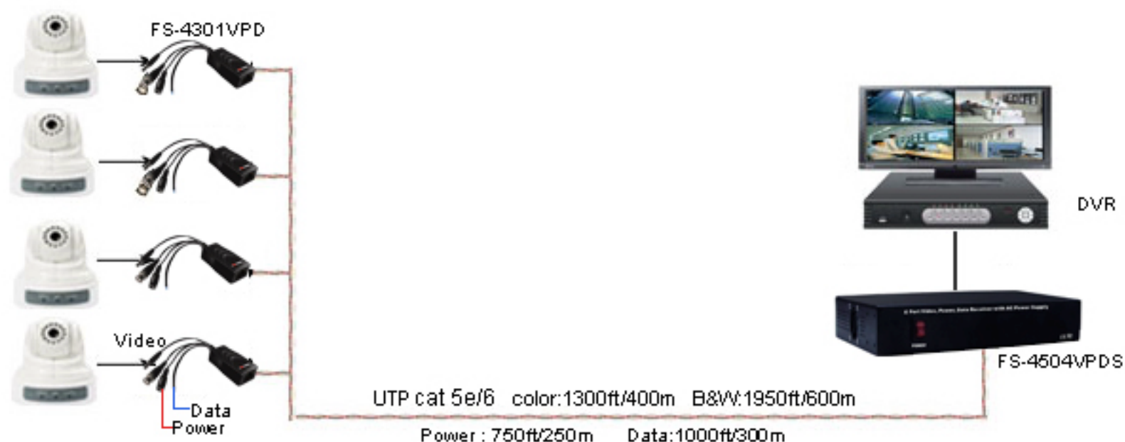
Diagram 2 FS-4301VPD + FS-4504VPDS (for 24VAC PTZ camera )
