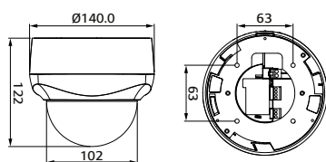
[ LND3220R_Side / Rear ]
