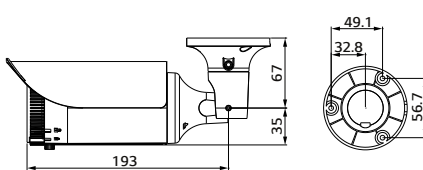
[ LNU3220R_Side / Rear ]
