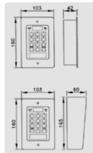
Art. VX 800NS/A Art. VX 900NS/A
