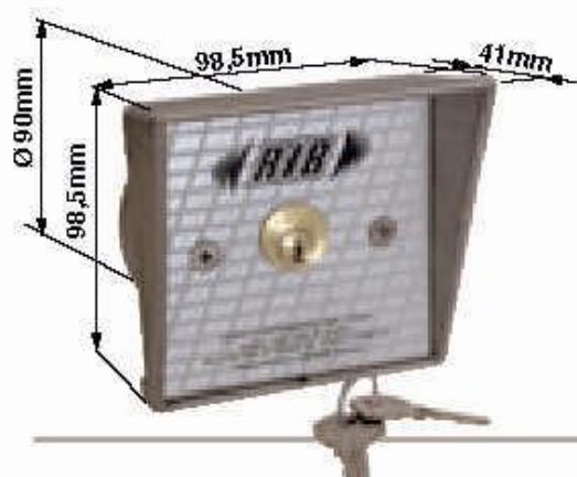
ACG1010 EMBEDDED open close IP44
