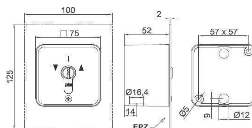
A encastrer flush mount
