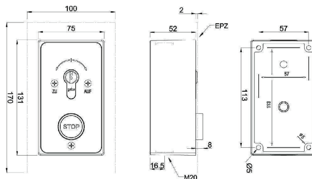
A encastrer / flush mount
