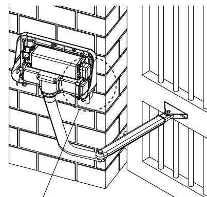
LEFT-HAND APROLI ELECTRIC MOTOR TERMINAL BOX
