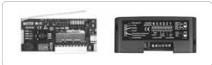
RECEIVER CARD TO MANAGE WIRELESS SYSTEM with connector - 12÷30V ac/dc code ACG6094 with terminal block - 12÷30V ac/dc code ACG6099
