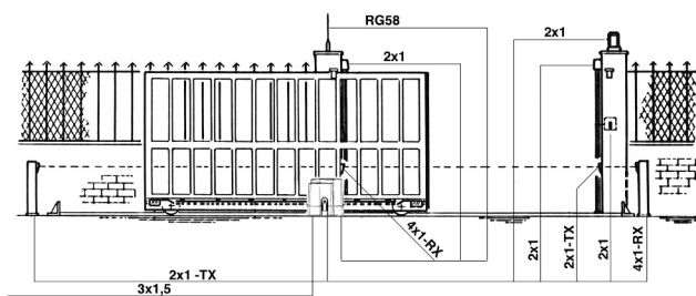
POWER SUPPLY
