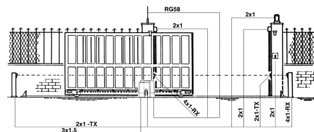
POWER SUPPLY
