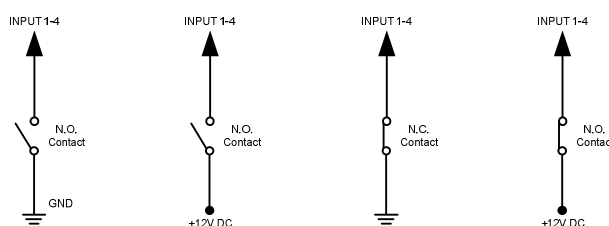
Figure 2: Output configuration
