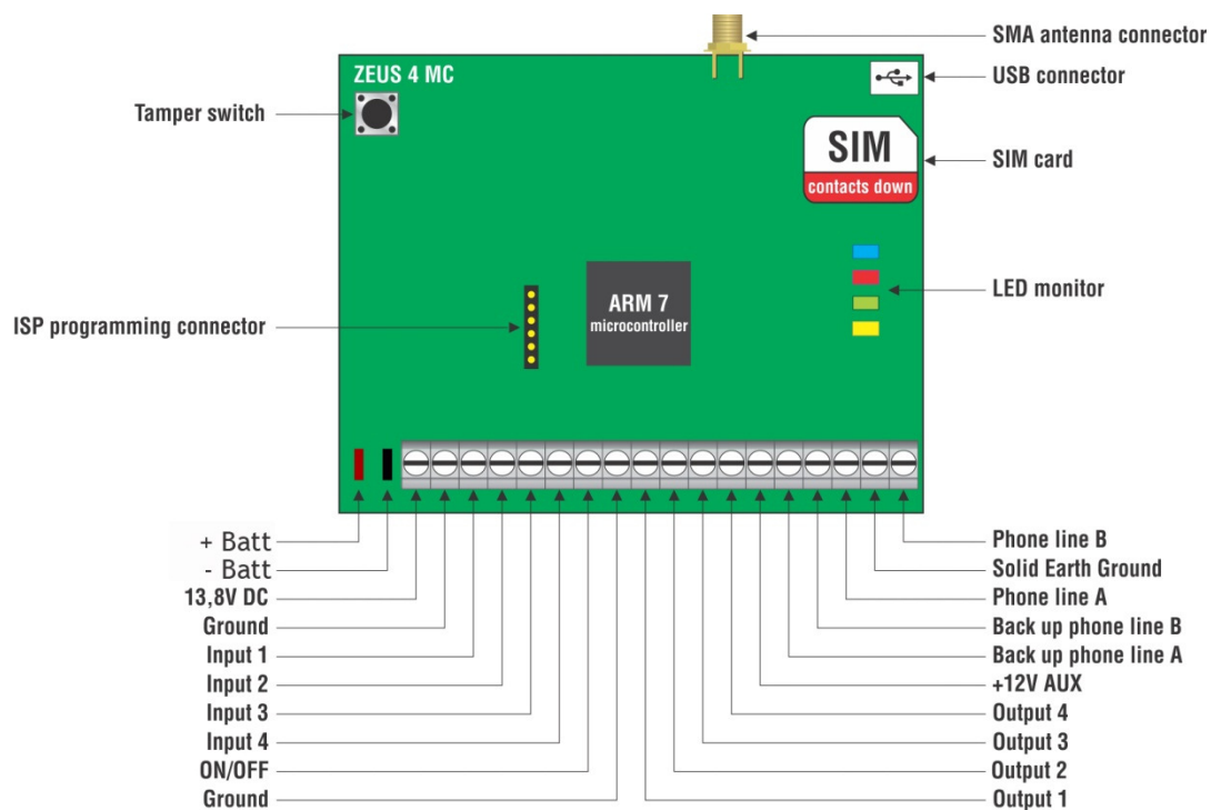
Figure 1: Connection diagram
