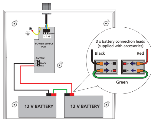
LOCATION OF 2 x 12 V BATTERIES AND CONNECTION OF BATTERY LEADS TO THE POWER SUPPLY PCB
