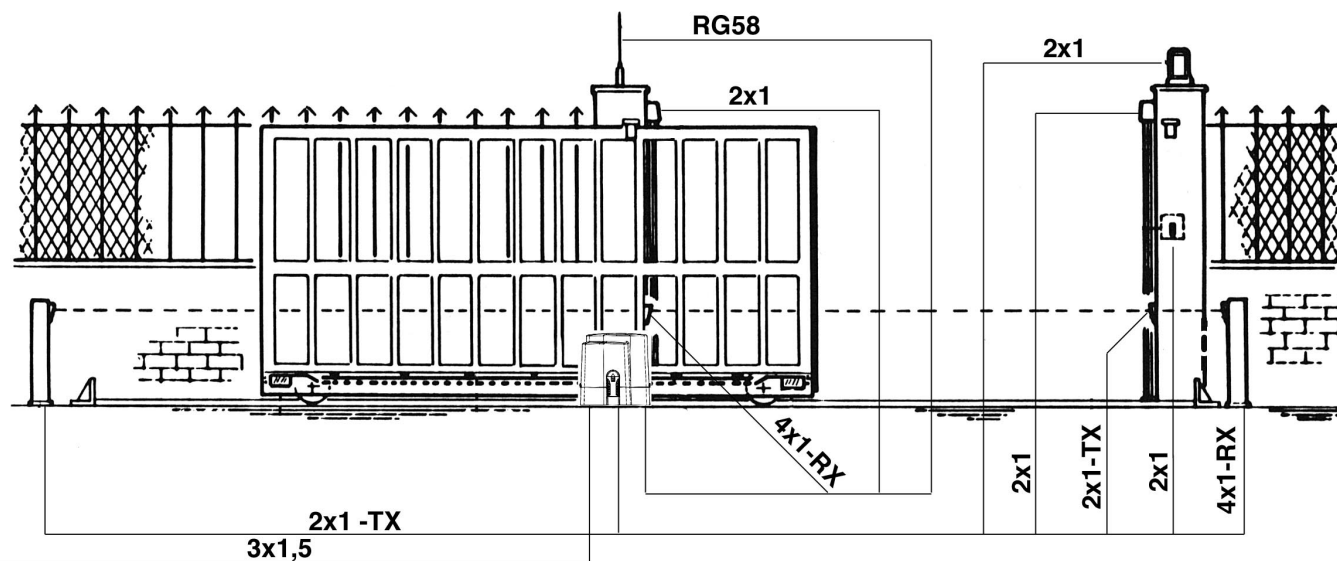
POWER SUPPLY
