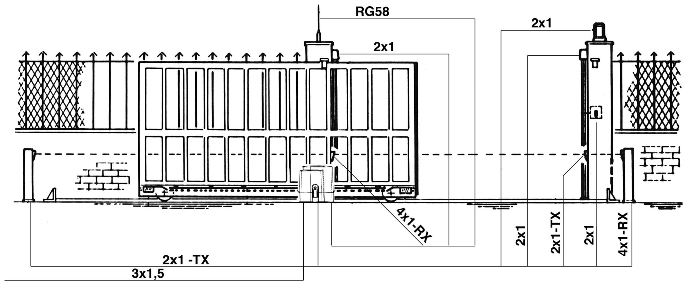
POWER SUPPLY
