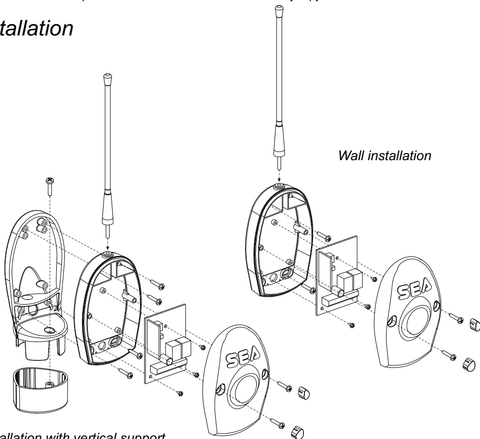
Installation with vertical support
