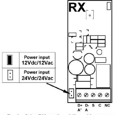
Back of the RX card, welding side Configuration of the contact to be used
