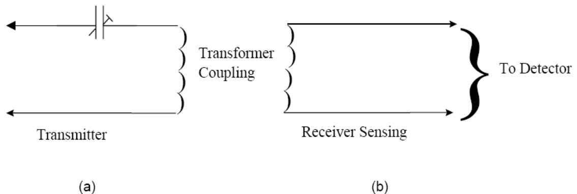
Figure 4.1: Transformer coupling
