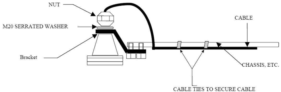
Figure 5.2: Recommended TRANSMITTER mounting details
