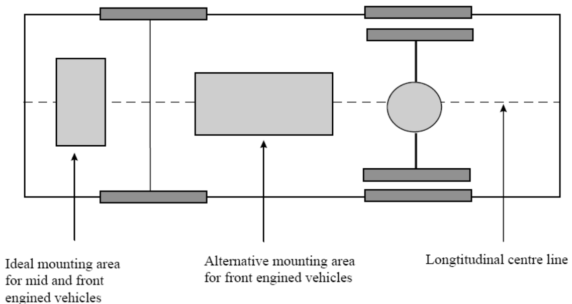
Figure 5.1: Underside view of vehicle
