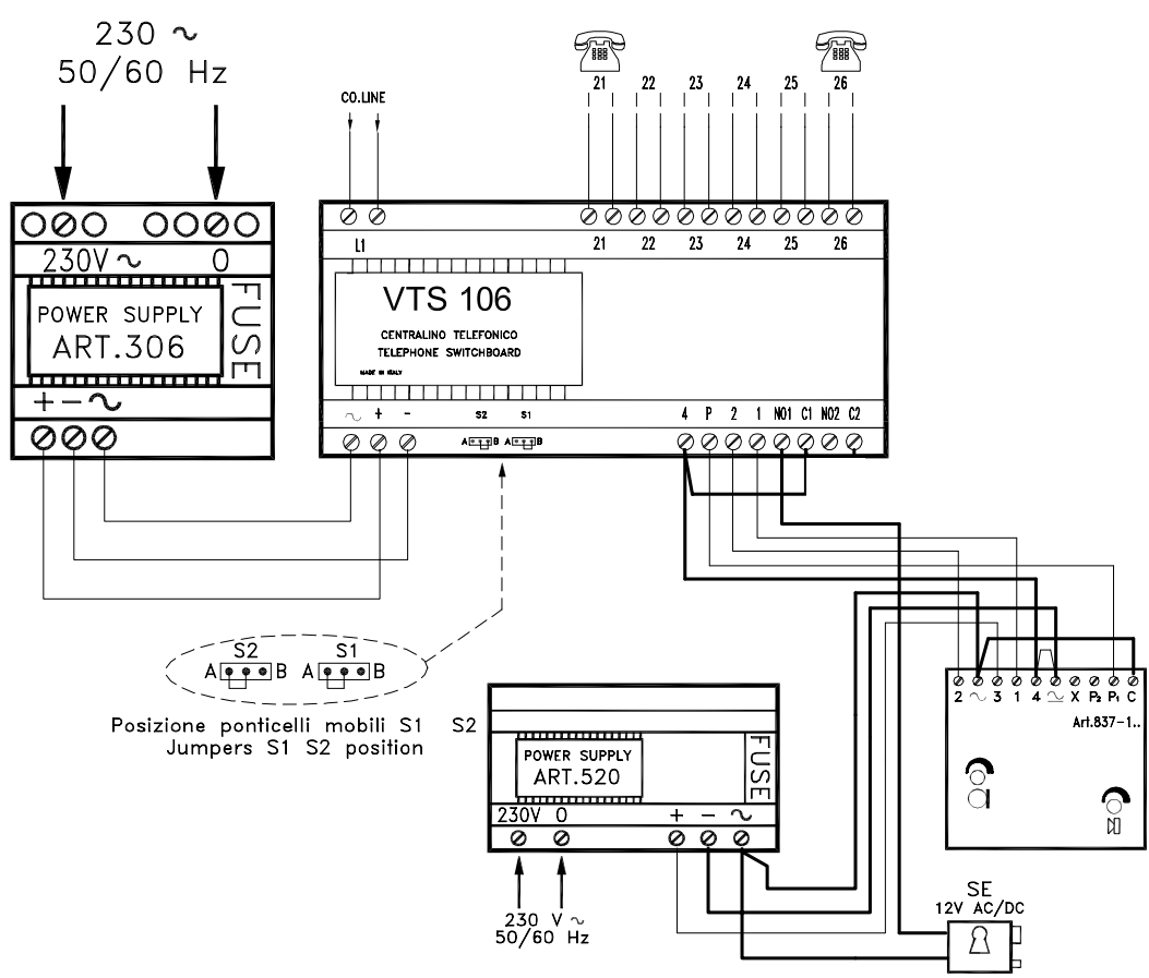
VTS 106 INTERCOM TELEPHONE SWITCHBOARD WITH ONE OUTDOOR STATION
