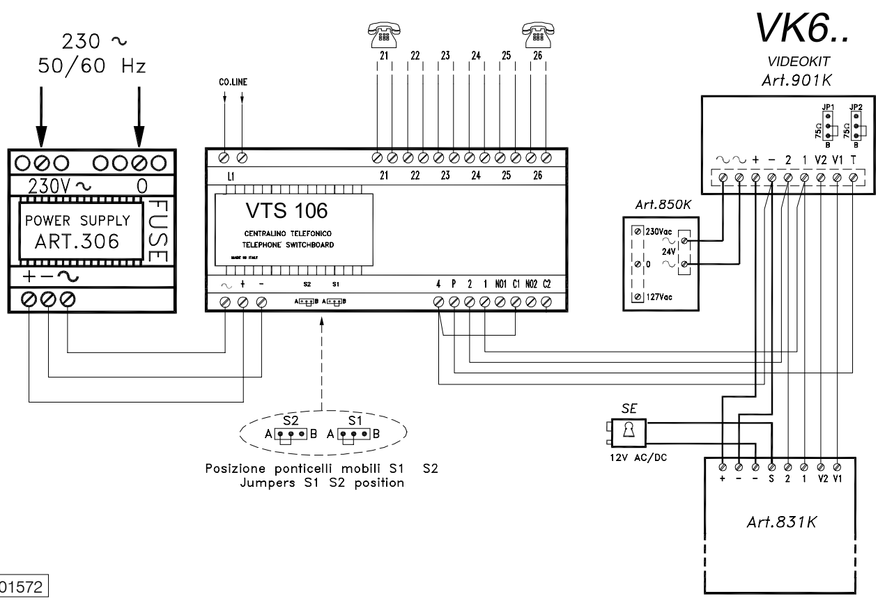
VTS 106 TELEPHONE SWITCHBOARD + VIDEOKIT VK6
