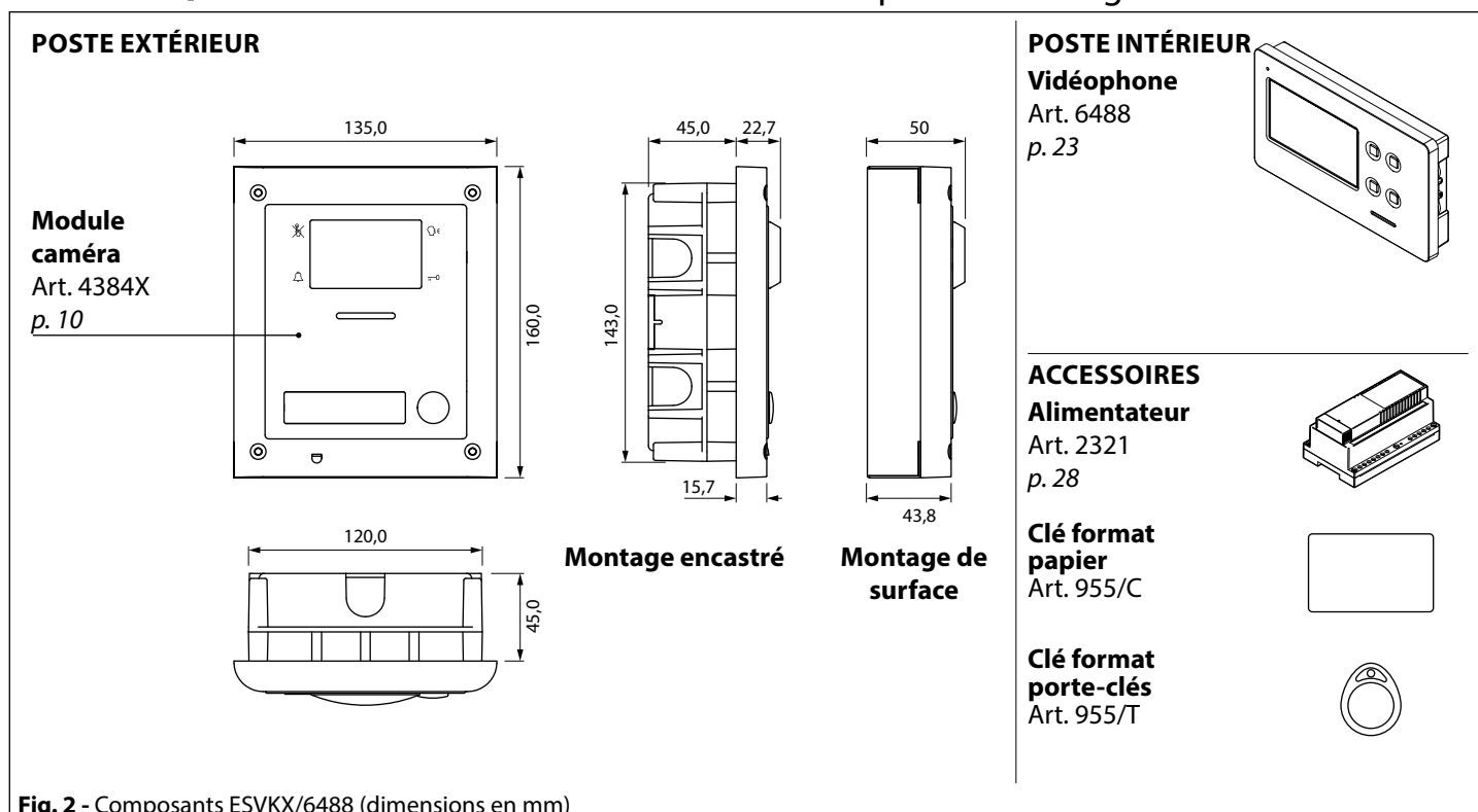
Fig. 2 - Composants ESVKX/6488 (dimensions en mm)
