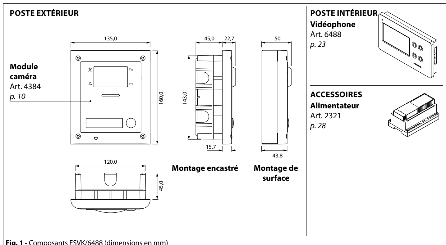
Fig. 1 - Composants ESVK/6488 (dimensions en mm)
