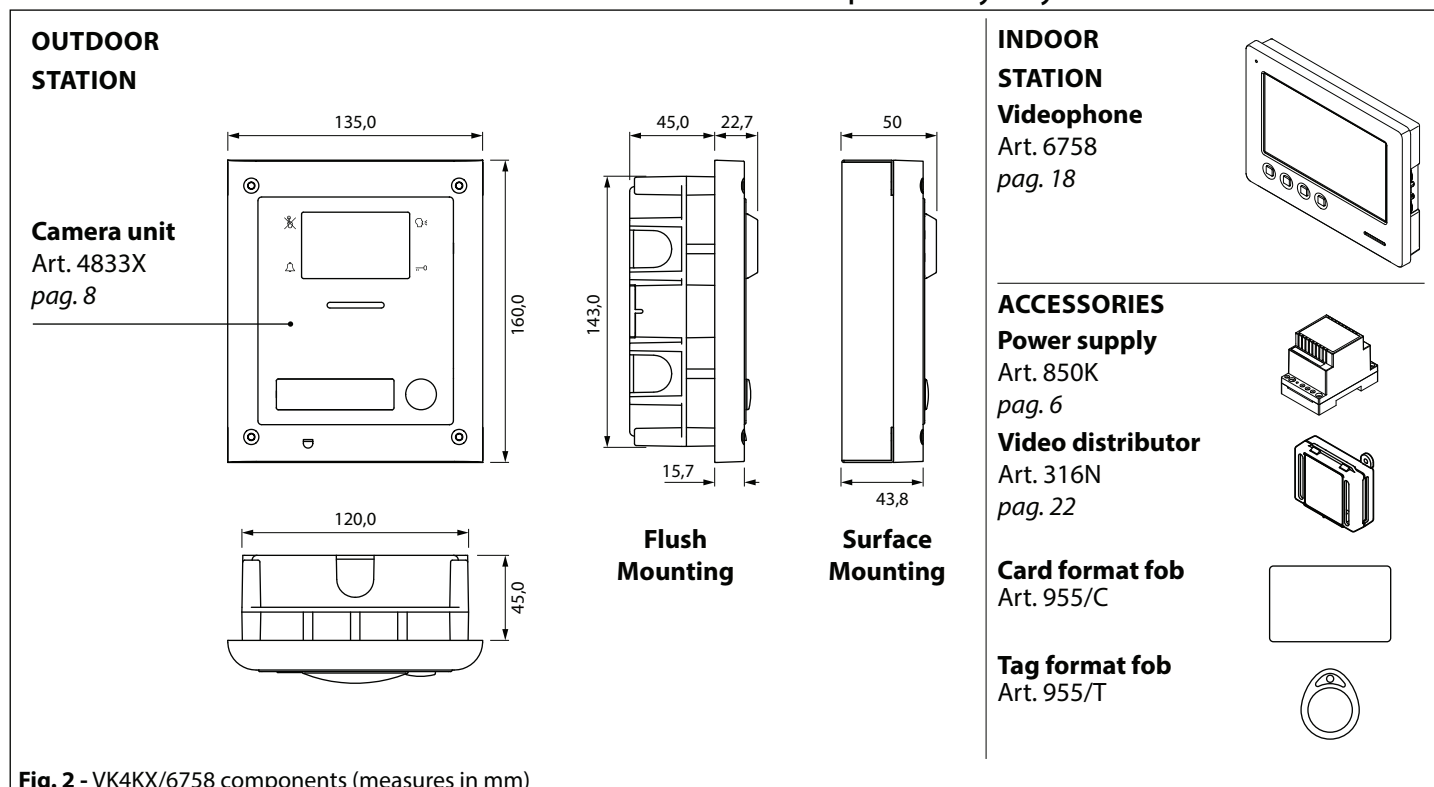
Fig. 2 - VK4KX/6758 components (measures in mm)
