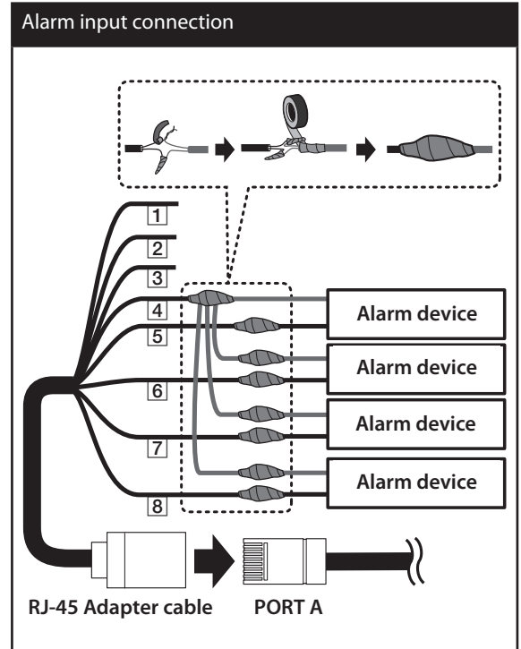
RJ-45 Adapter cable
